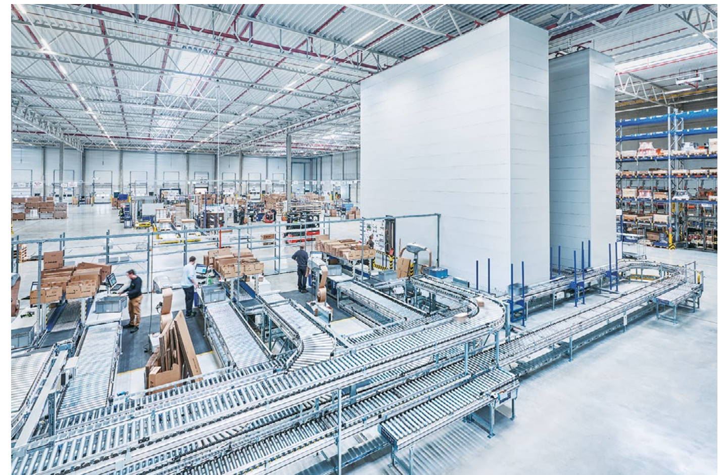
Vertical Buffer Modules Kardex Miniload-in-a-Box* with automated conveyor connection
